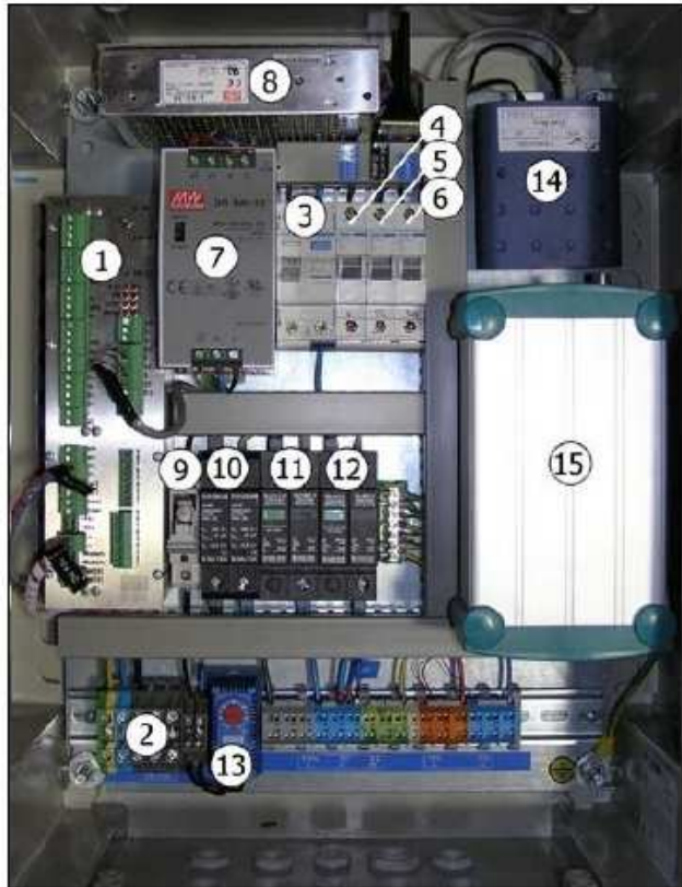
Components of the internal outfit of the meteorological station
